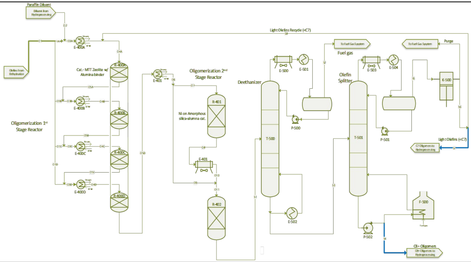
Figure 27- Oligomerization of Olefins to Oligomers PFD
