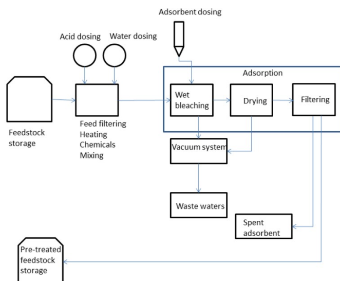
Figure 7: HEFA feedstock pretreatment
