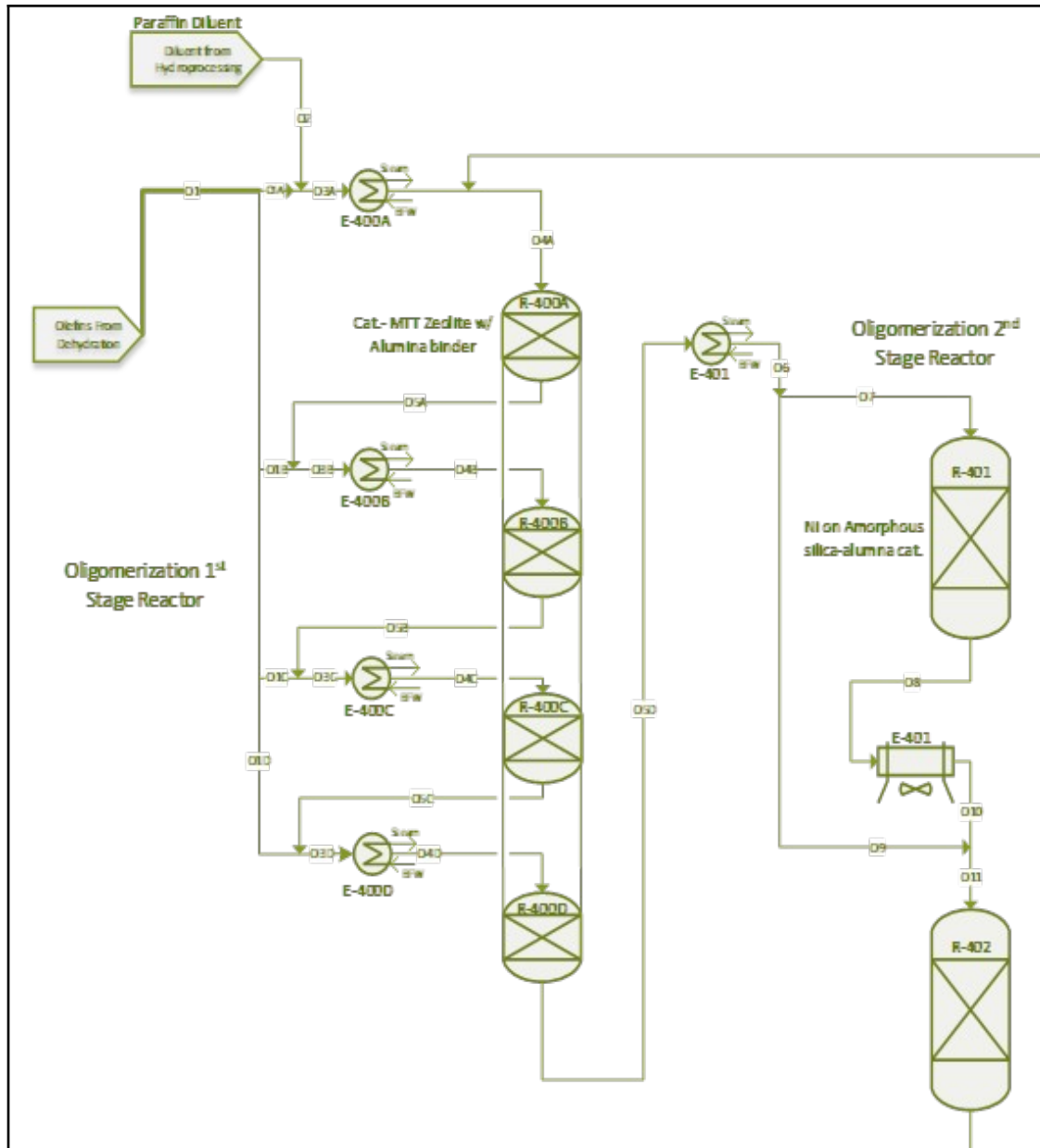
Figure 28- Oligomerization Reactor Section
