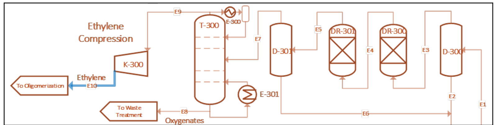
Figure 26- Ethylene Purification Section
