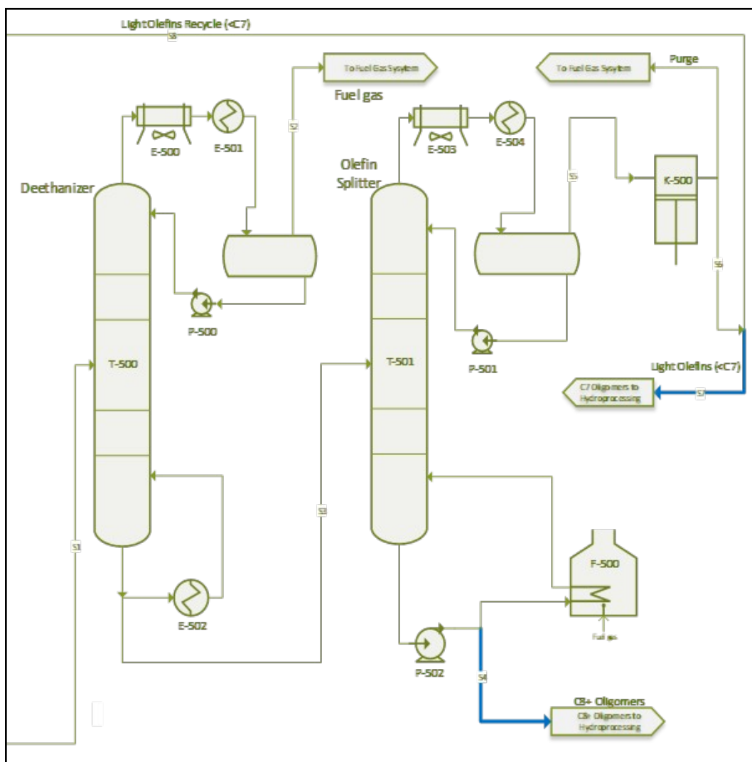
Figure 29- Olefin Separation Section
