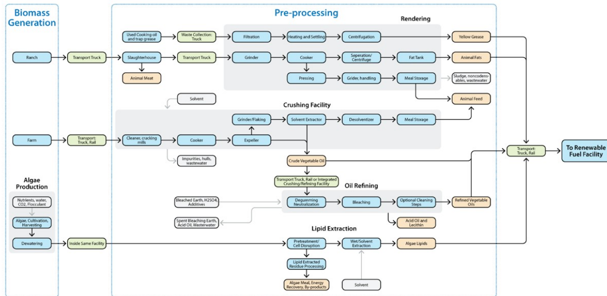
Figure 9: HEFA block flow diagram part 1
