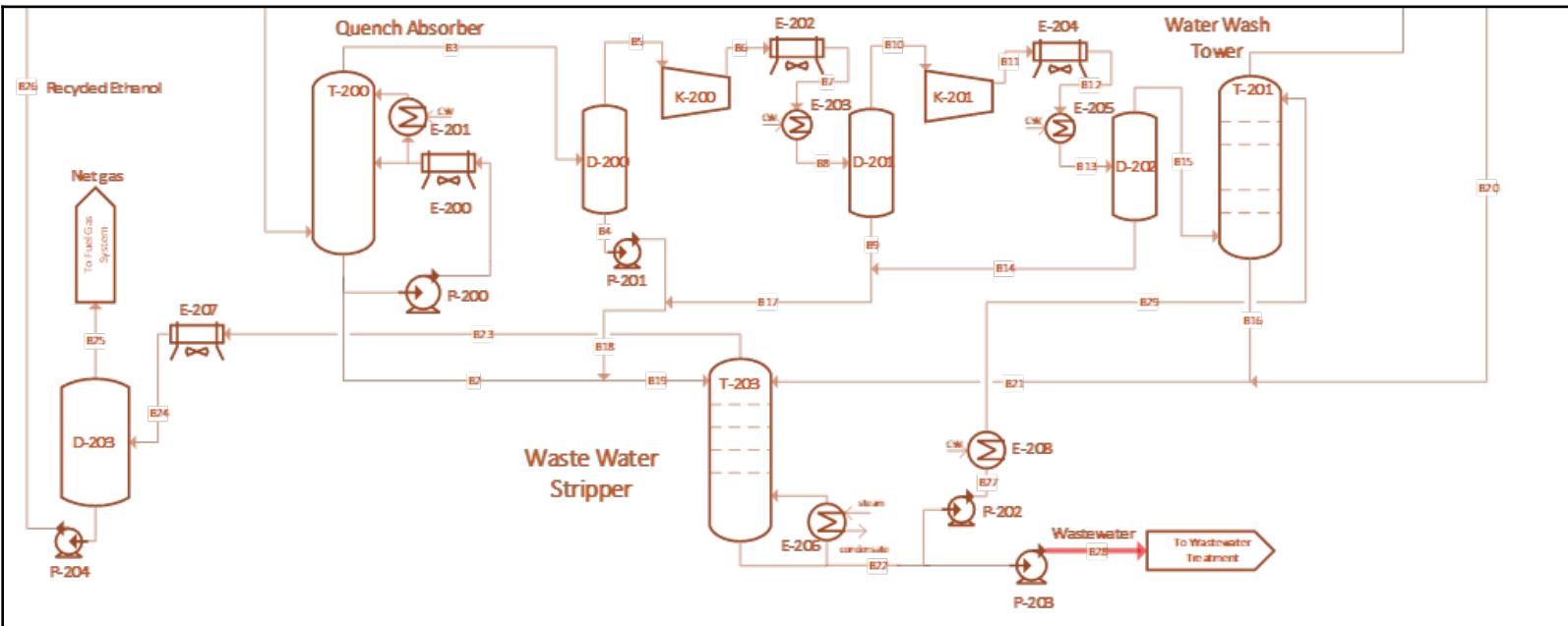
Figure 25- Byproduct Removal Section
