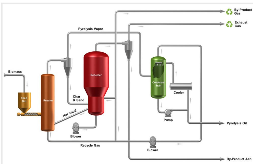
Figure 12: Pyrolysis Block flow diagram
