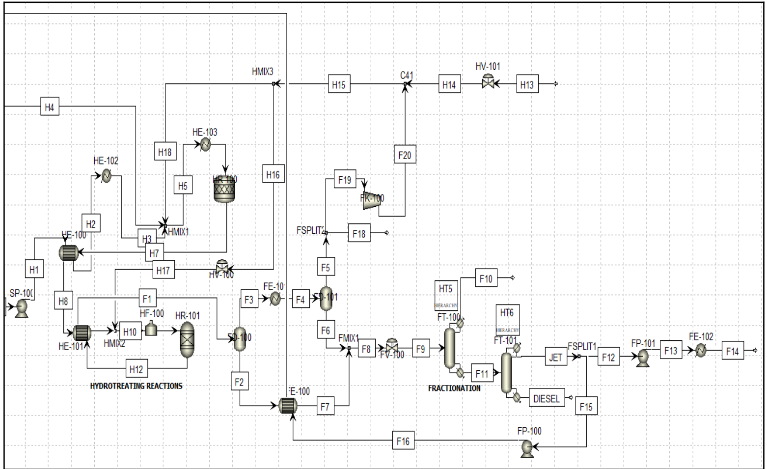
Figure 35- Hydroprocessing of Oligomers to Jet Fuel Simulation PFD
