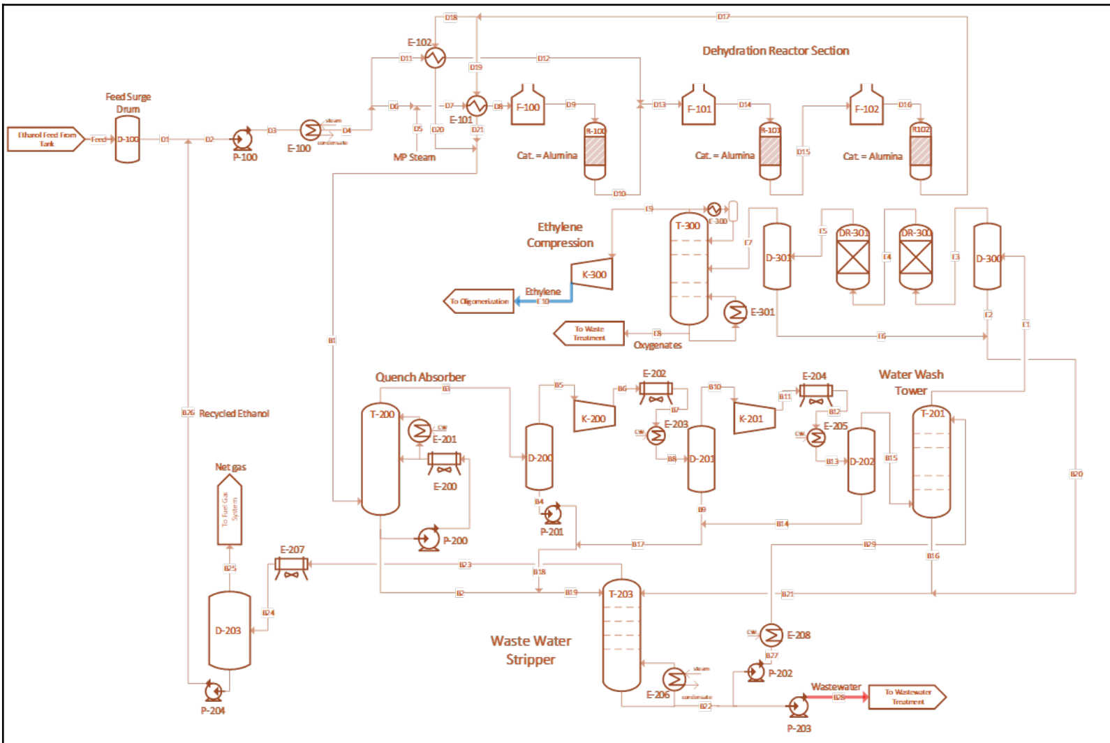
Figure 23- Dehydration of Ethanol to Ethylene PFD
