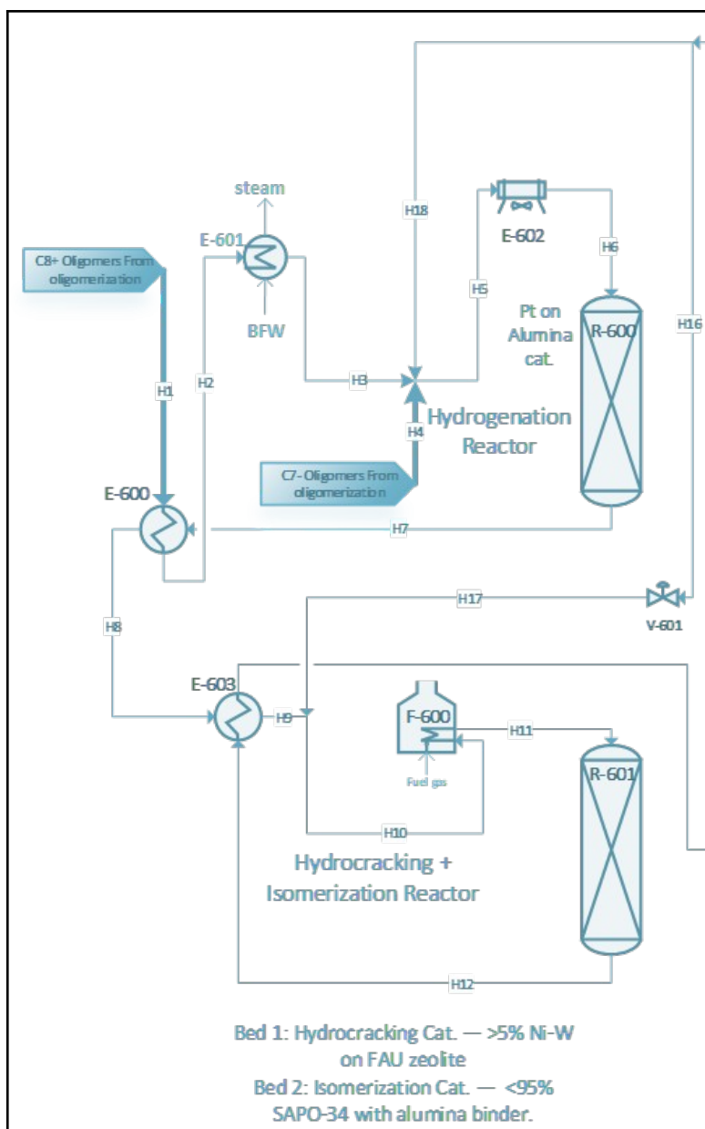
Figure 31- Hydroprocessing Reactions Section
