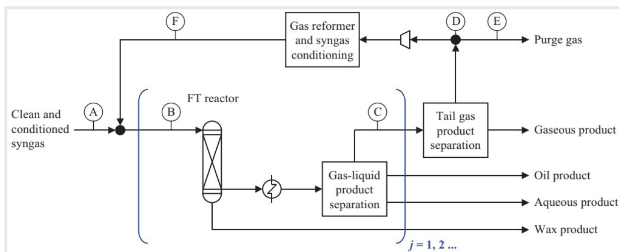
Figure 11: gFT block flow diagram
