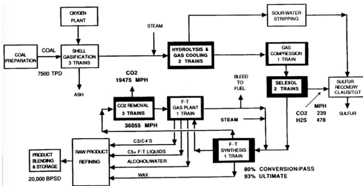
Figure 15: slurry reactor bfd
