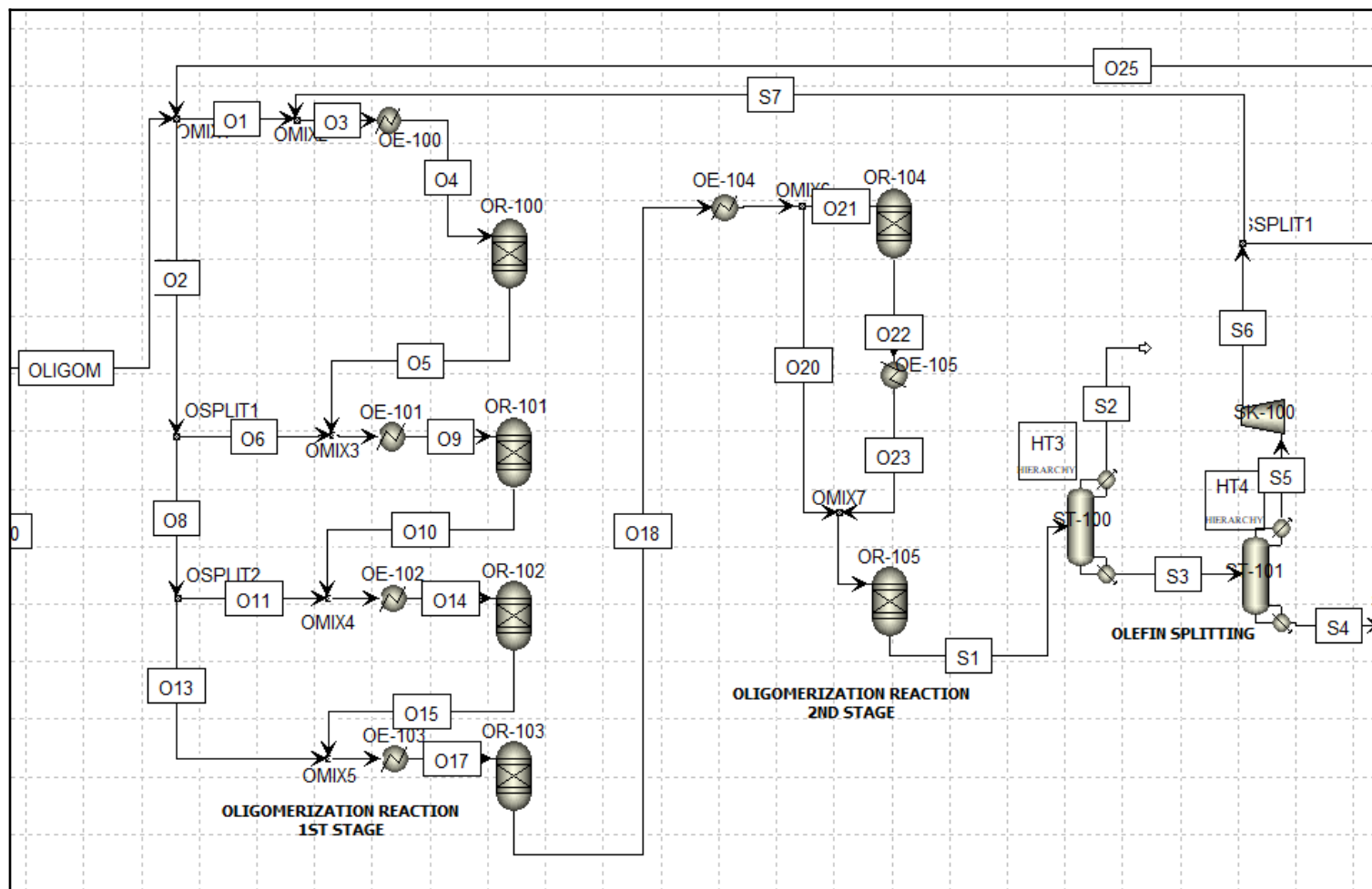
Figure 34- Oligomerization of Ethylene to Oligomers Simulation PFD
