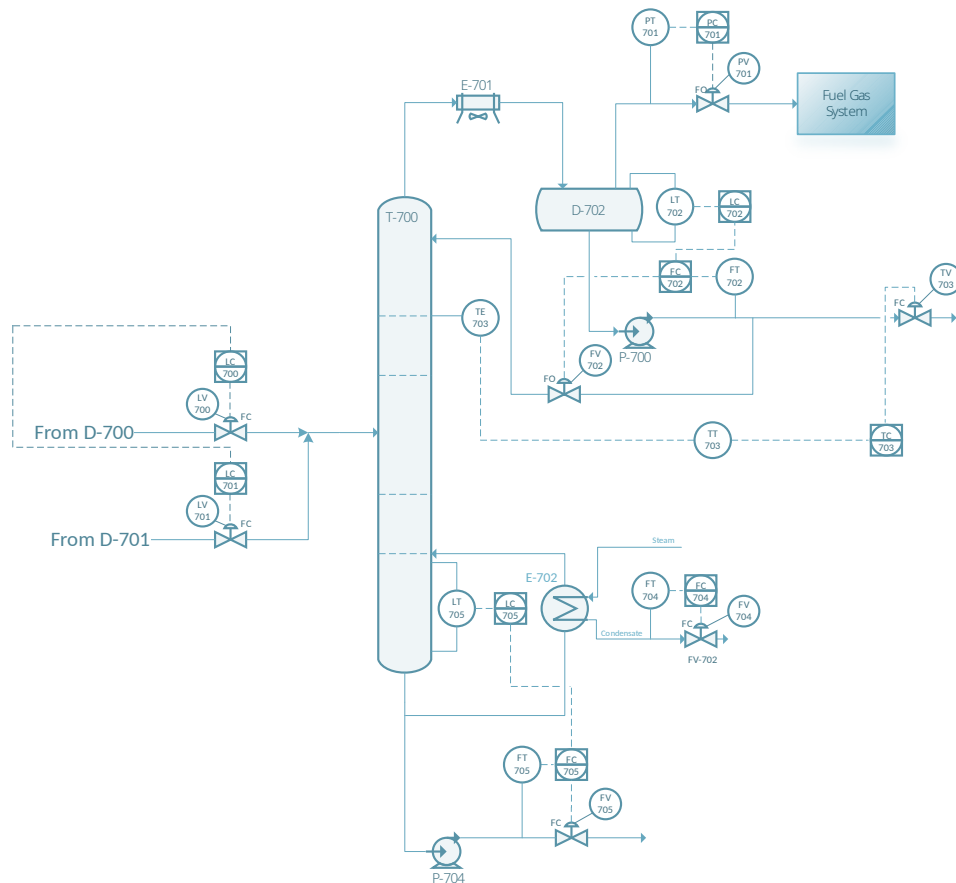
Figure 18- Process Control Loop on Fractionator Before HAZOP
