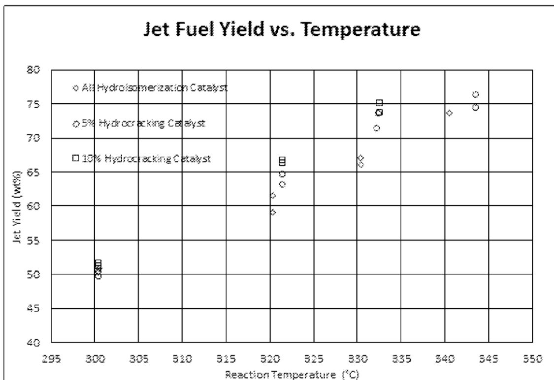
Figure 17- Jet Fuel Yield vs. Temperature [18]
