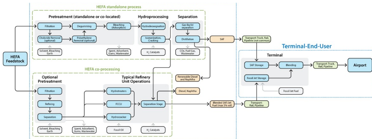
Figure 10: HEFA BFD part 2
