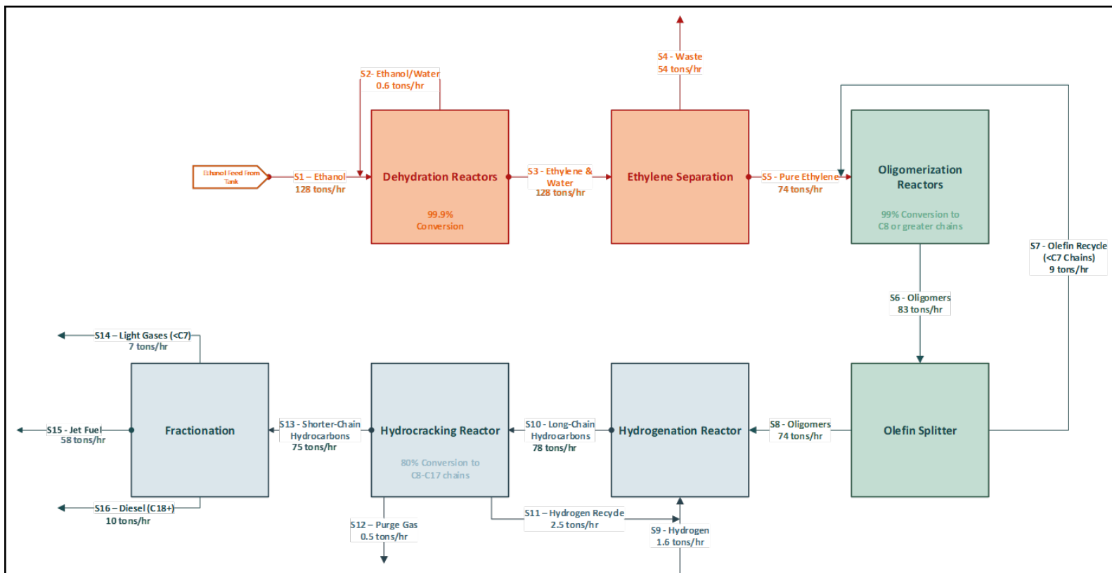
Figure 22- Ethanol to Jet Fuel BFD
