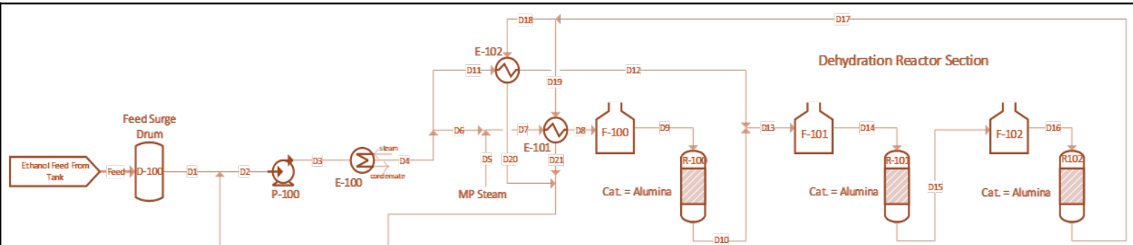
Figure 24- Dehydration Reactor Section
