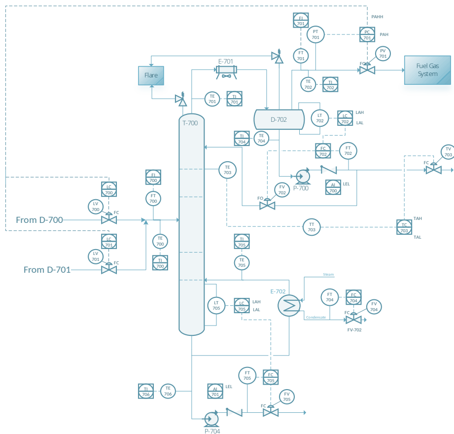
Figure 19- Process Control Loop on Fractionator After HAZOP
